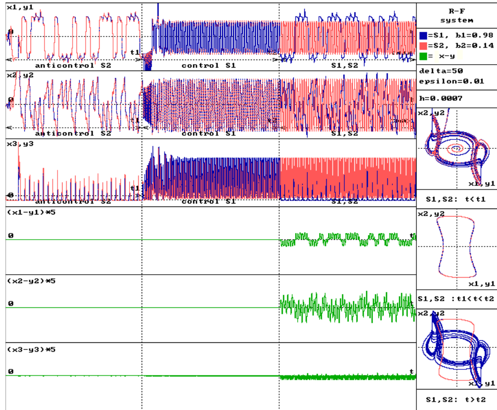
Figure 3: The CA algorithm applied to R-F system (13) for \delta = 50 and \epsilon = 0.01 .
