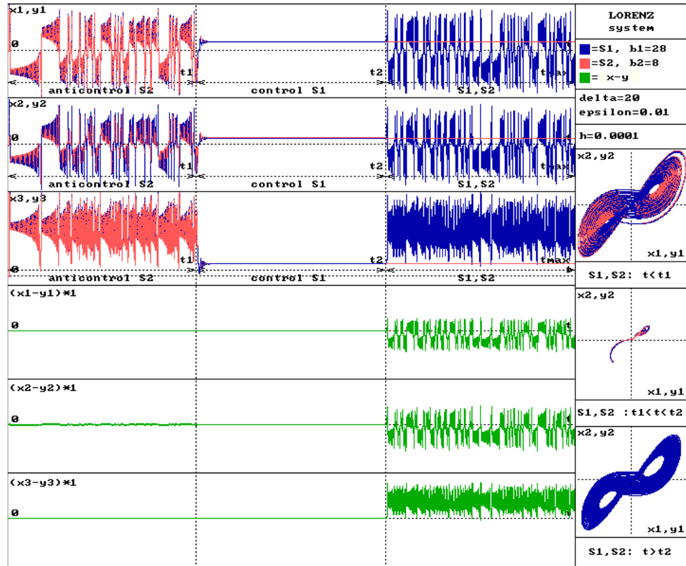
Figure 1: The CA algorithm applied to Lorenz system (11) for \delta = 20 and \varepsilon = 0.01 .
