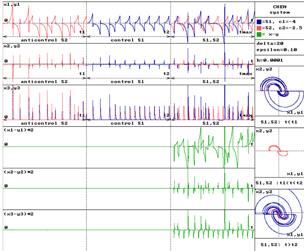
Figure 2: The CA algorithm applied to Chen system (12) for \delta = 20 and \epsilon = 0.1 .
