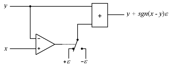
Figure 4: Circuitry implementation of CA algorithm.
